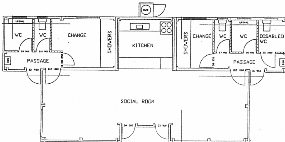
SPORTS PAVILION BUILT ON TOP OF A 6 METER DEEP RUBBISH TIP
