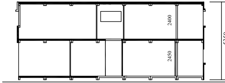
SECTION C
