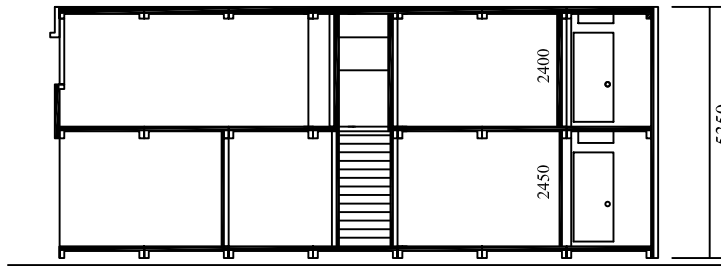
SECTION A
