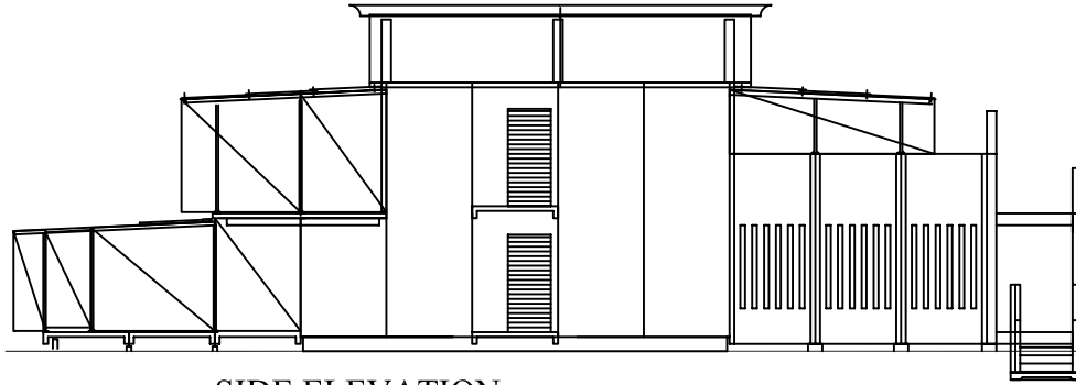
SIDE ELEVATION
