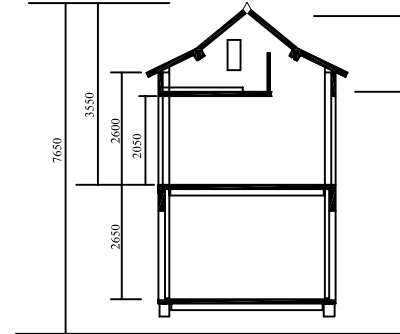
SECTION B
