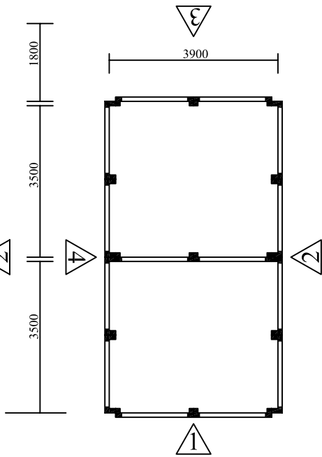
PLAN TOP FLOOR
