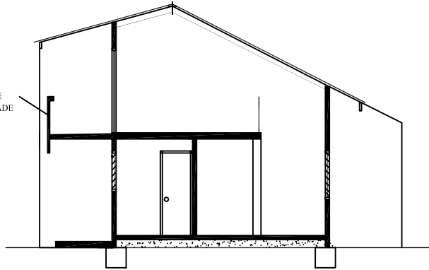
SECTION B
