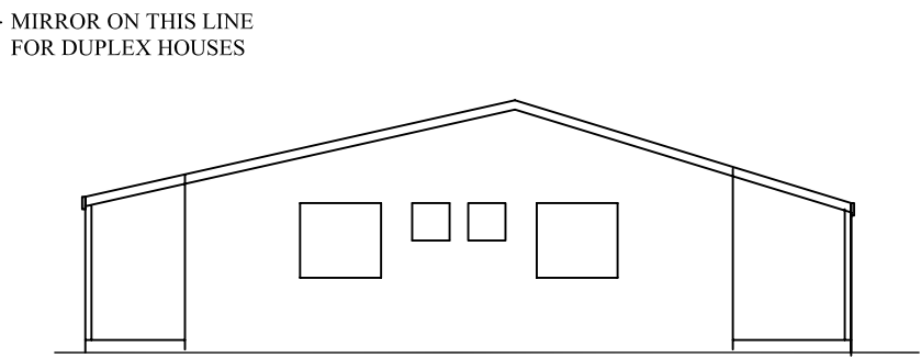
SIDE ELEVATION
