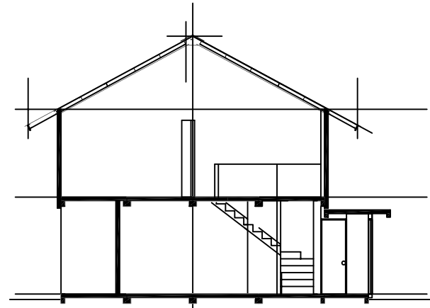
LONG SECTION
