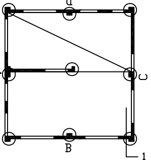
PLAN - FULL HOUSE - STRUCTURE
