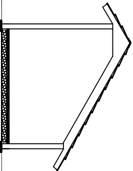
SECTION 2
